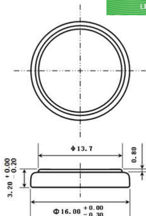
Dimension Drawing
